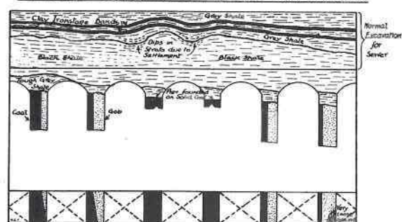
GEOLOGICAL SECTION & PLAN OF OLD COAL WORKINGS.
