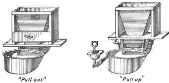
Moule's patent earth-closet
