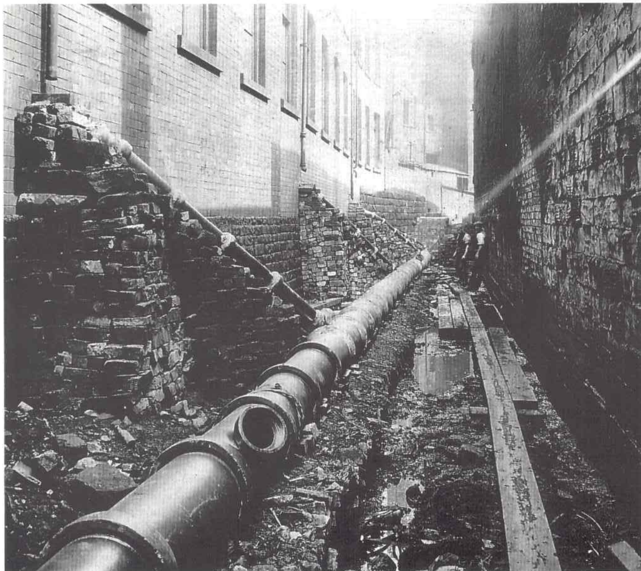
Sewer construction in an old goit at Warehouse Hill, 1906
