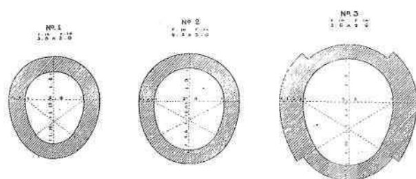
Egg shaped sewer cross-sections
