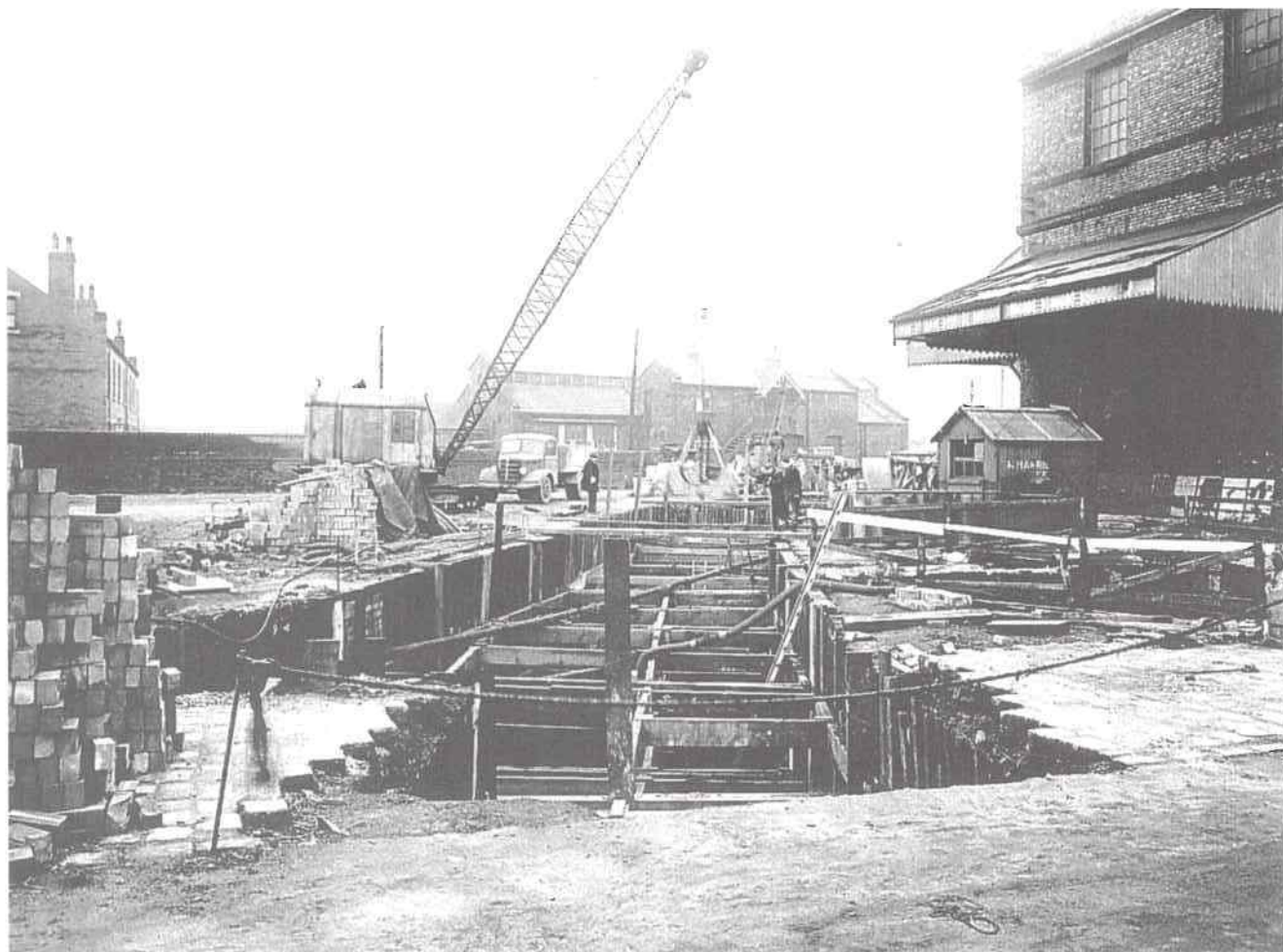
Low Level Sewer diversion work at Hunslet goods station, 1951
