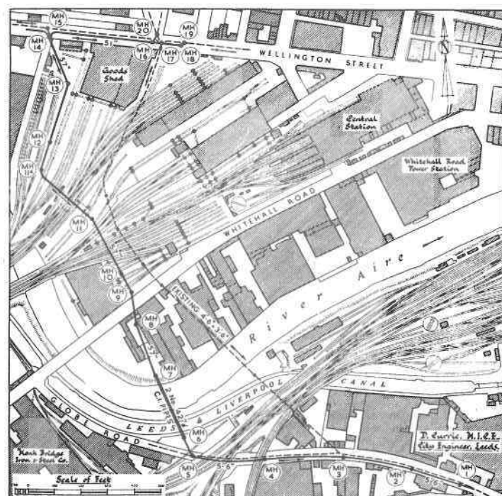
Fig. 7 Plan showing replacement of the old Low Level Sewer near Globe Road, 1961
