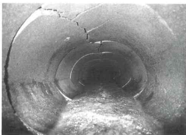
CCTV can reveal badly fractured sewers (Garforth, 1970's)
