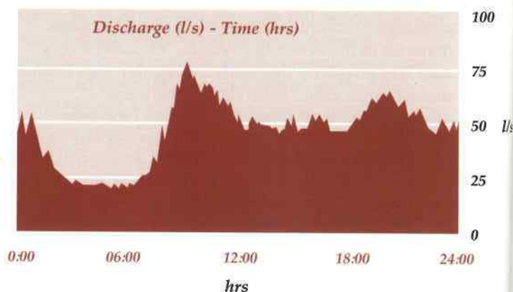
Fig. 8 Variation of dry weather flow during the course of a day. (High Level Sewer near Kirkstall Abbey)
